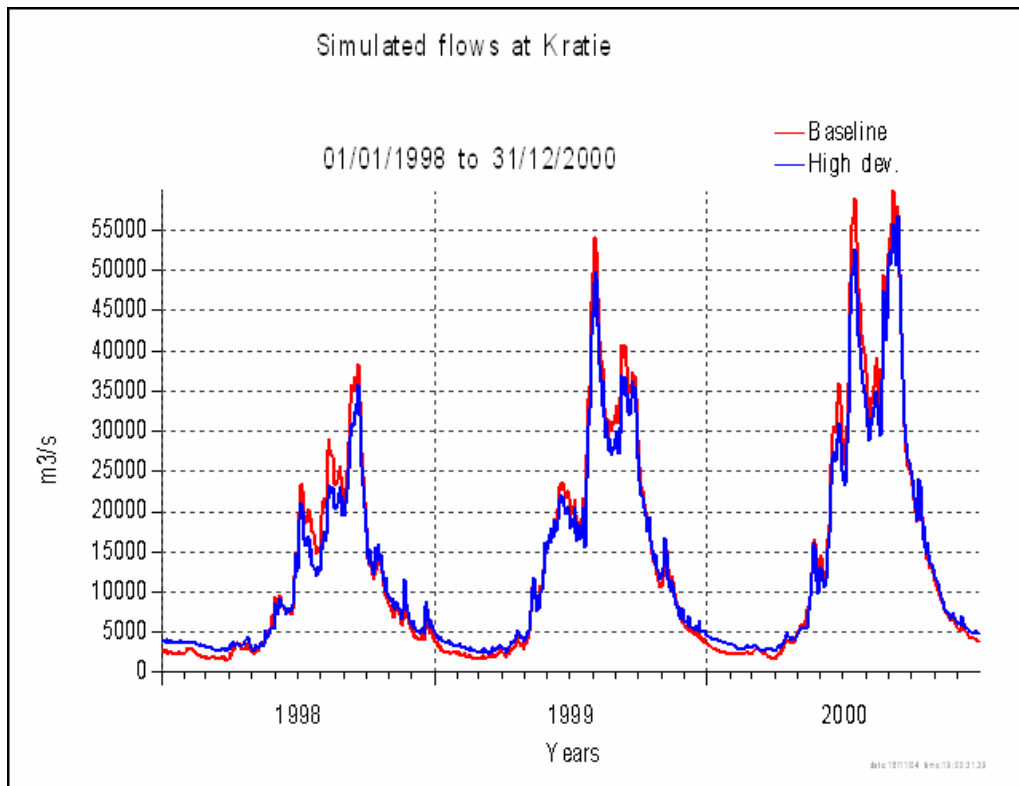
Figure 3 Simulated flows at Kratie
